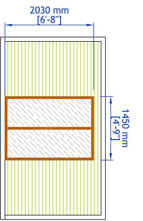
Front Elevation
