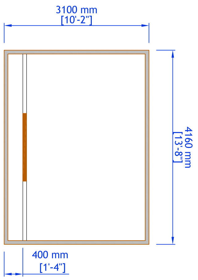
Plan
